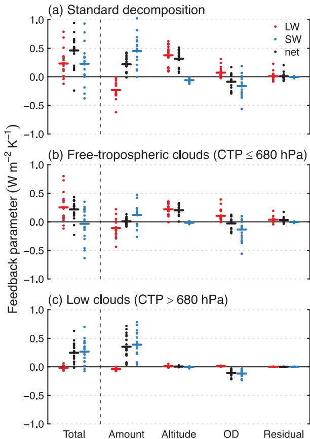
FIGURE 2 | Global-mean longwave (red), shortwave (blue), and net (black) cloud feedbacks decomposed into amount, altitude, optical depth, and residual components for (a) all clouds, (b) free-tropospheric clouds only, and (c) low clouds only, defined by cloud top pressure. Multimodel-mean feedbacks are shown as horizontal lines. Results are based on an analysis of 11 CMIP3 and 7 CMIP5 models 26 ; the CMIP3 values do not account for rapid adjustments. Model names and total feedback values are listed in Table S2. (Reprinted with permission from Ref 26. Copyright 2016 John Wiley and Sons)
