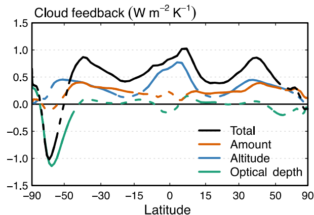
FIGURE 4 | Zonal-, annual-, and multimodel-mean net cloud feedbacks in a set of 11 CMIP3 and 7 CMIP5 models (Table S2), plotted against the sine of latitude, and partitioned into components due to the change in cloud amount, altitude, and optical depth. Curves are solid where 75% or more of the models agree on the sign of the feedback, dashed otherwise. (Reprinted with permission from Ref 26. Copyright 2016 John Wiley and Sons)
