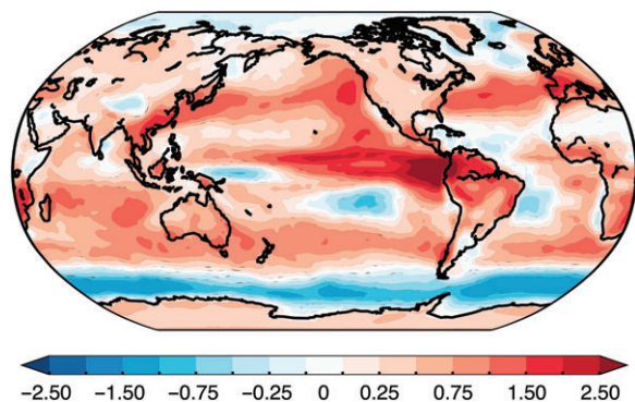
FIGURE 3 | Spatial distribution of the multimodel-mean net cloud feedback (in \text{W m}^{-2} per K surface warming) in a set of 11 CMIP3 and 7 CMIP5 models subjected to an abrupt increase in \text{CO}_2 (Table S2). (Reprinted with permission from Ref 26. Copyright 2016 John Wiley and Sons)
