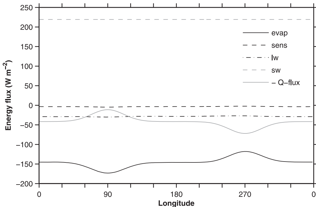
FIG. 3. Surface energy fluxes of the reference simulation vs longitude averaged within 8^\circ of equator. Here, “lw” and “sw” refer to the net longwave and shortwave radiative fluxes at the surface, respectively.
