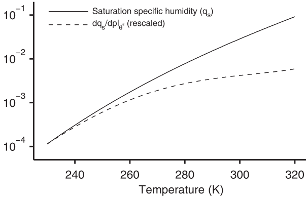
FIG. 6. Saturation specific humidity (solid) and the rescaled moist-adiabatic derivative of saturation specific humidity dq_s/dp|_{\theta^*} (dashed). Both quantities are evaluated at a pressure of 800 hPa. The moist-adiabatic derivative of saturation specific humidity has been rescaled by a dimensional constant so that it agrees with the saturation specific humidity at the lowest temperature shown. At 280 K, the fractional rate of increase in saturation specific humidity is 6.9\% \text{ K}^{-1} , compared with 3.0\% \text{ K}^{-1} for the moist-adiabatic derivative of saturation specific humidity.
