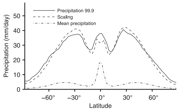
FIG. 1. The 99.9th percentile of daily precipitation (solid) and mean precipitation (dash-dotted) in the reference simulation ( \alpha = 1 ). The precipitation extremes scaling (4) is also shown (dashed), multiplied by a constant of proportionality of 3.5 so that it agrees with the 99.9th percentile in the global mean. Statistics shown here and in the following figures are based on zonal and time averages. Deviations from symmetry between the hemispheres are indicative of sampling error.
